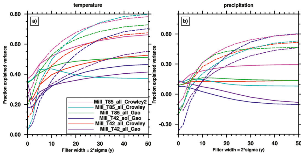
FIG. A1. Percentage of explained variance from (a) temperature and (b) precipitation estimates using regression values generated with unfiltered data (solid lines) and with filtered data (dashed lines). Different colors correspond to different simulations.
